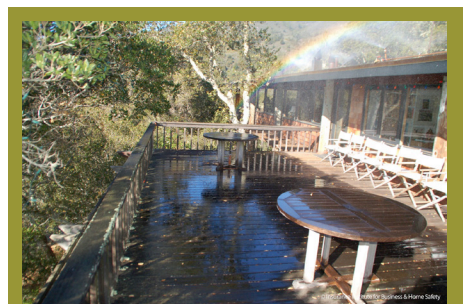
Photo 3. Roof-edge mounted sprinkler. Note these sprinklers did not deliver water in the near-home area. With this scenario, a sufficient number of wind-blown embers would have to be quenched in order to avoid ignition of the siding and decking in this zone, particularly at the deck-to-wall intersection.
